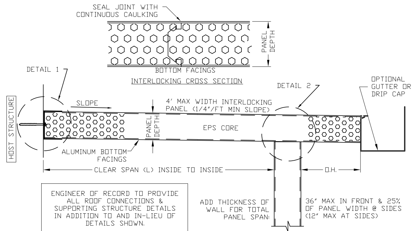
EPS ROOF PANEL/ SPAN DESCRIPTION
